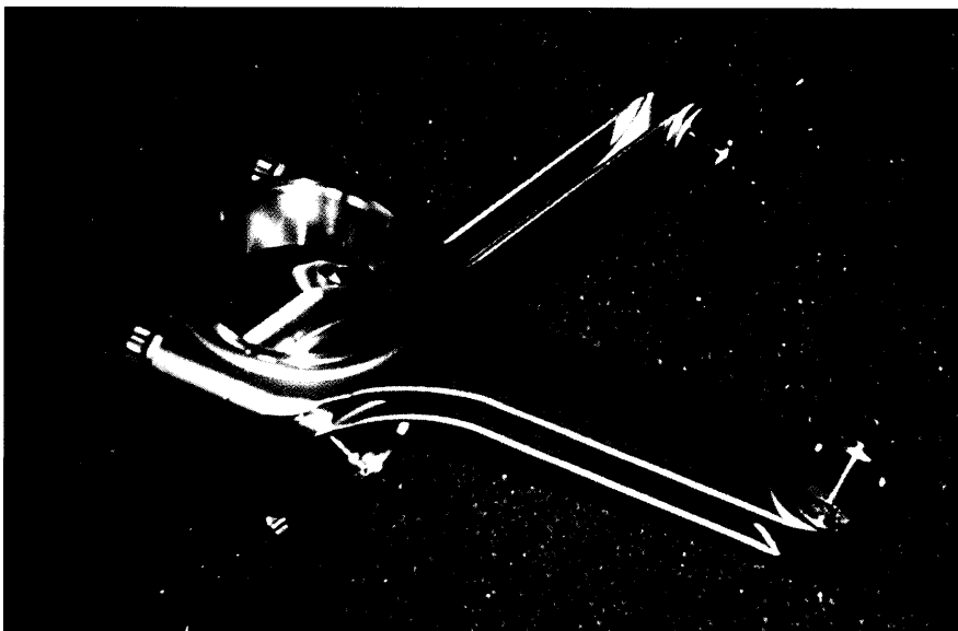
Connecting rods usually fail in fatigue. These lightweight, forged 300M steel connecting rods use cryogenic processing to resist the forces generated by an engine turning over 9000 rpm.
