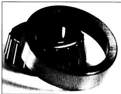
Fig. 6 — Cryogenic processing of ball and roller bearings increases their resistance to contact fatigue and increases life.
