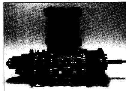
Fig. 4 — Jerico Performance Products is one of the racing component manufacturers that has recognized the value of cryogenic processing in extending component life. All gears, shafts, dogs made by Jerico are now cryogenically treated. In the year 2000, two thirds of the Winston Cup (NASCAR's premier series) race winners used transmissions made by Jerico.
