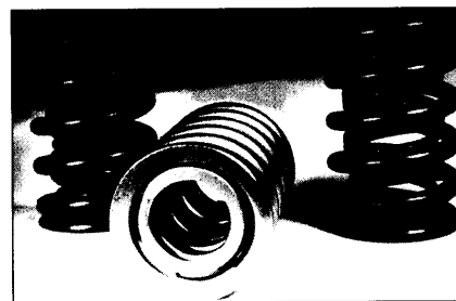
Fig. 3 — Valve springs show dramatic improvement in fatigue life, lose less preload, and show a smaller loss of spring constant when cryogenically processed. Vibrational characteristics are also changed.
